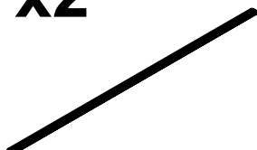
Profile tube 30x60x3 L=2502,5 2000521 p4
