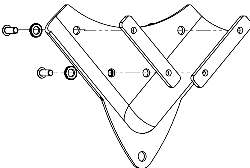
Corner for platform 30 mm 3085217
