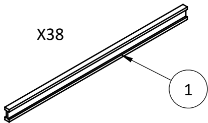
Beam, 074930 VT20K, L=3300, Peri 2001057
