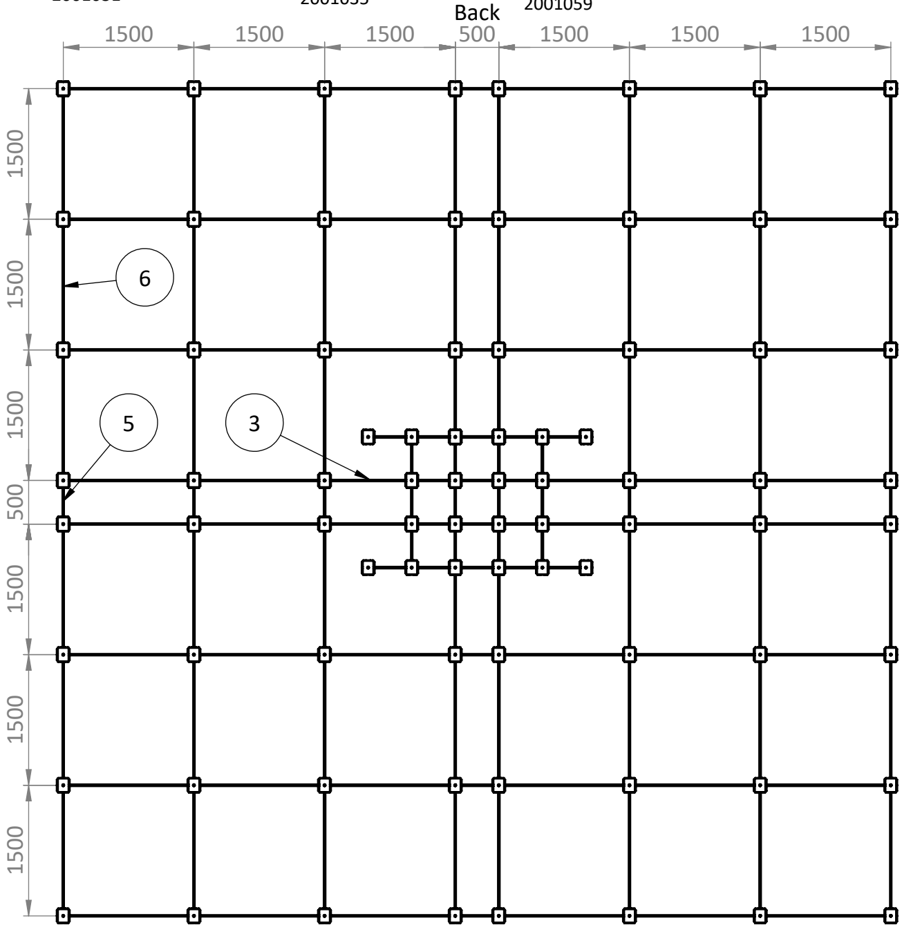
X40 Support beam L=500 2001031
